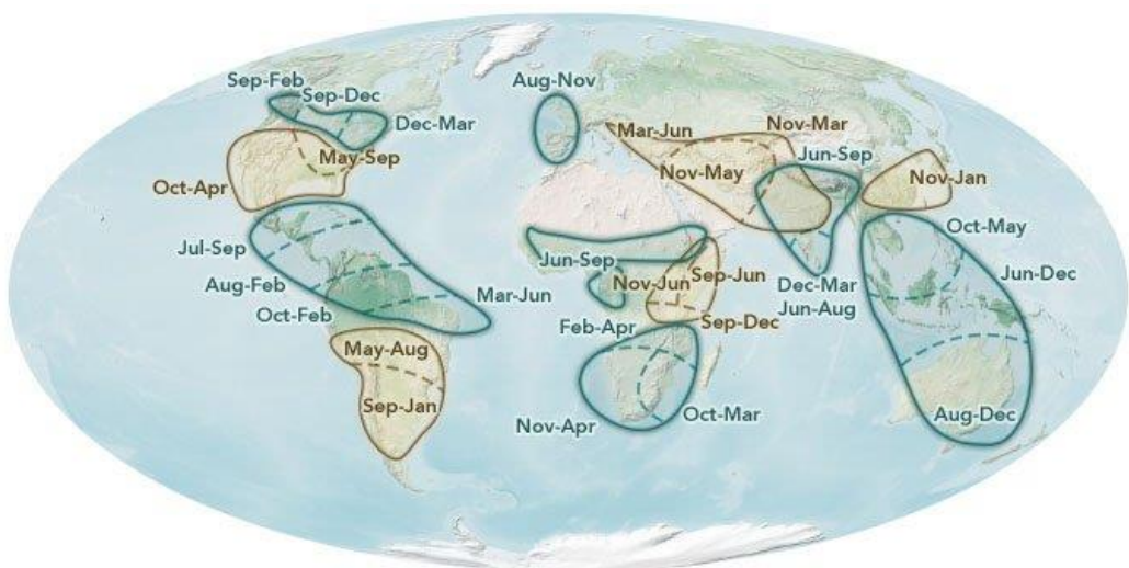
La Niña Heralds Different Conditions at Different Times
